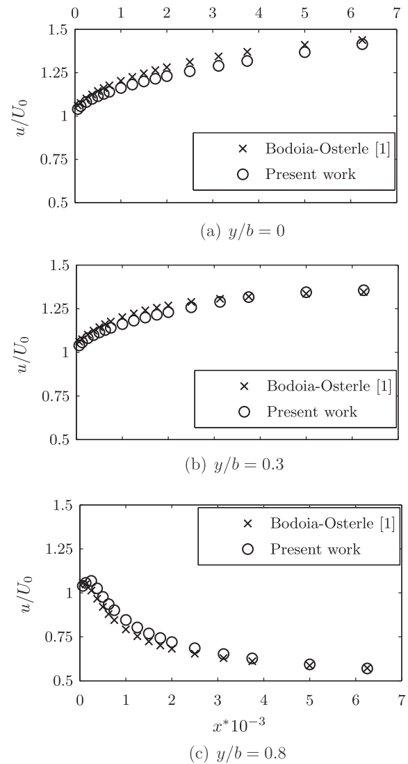
Fig. 3. Evolution of the axial velocity component for Newtonian fluid at three transversal positions.
